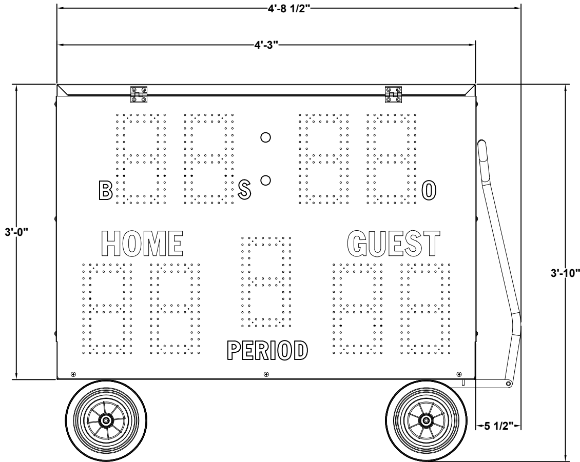
PSO-6900/PSO-6900-BATT (USING 12”H AMBER LED OUTDOOR DIGITS) FACE VIEW
