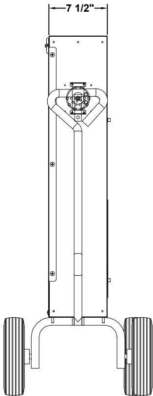
END VIEW
