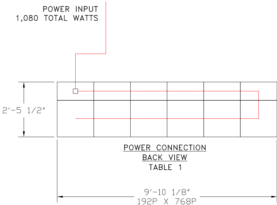
CST-103E, 3.9MM 192H X 768L INDOOR FRONT SERVICE SINGLE-FACE FULL-COLOR DIGITAL VIDEO DISPLAY POWER CONNECTION BACK VIEW
