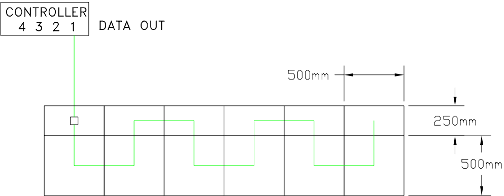
DATA CONNECTION BACK VIEW TABLE 1
