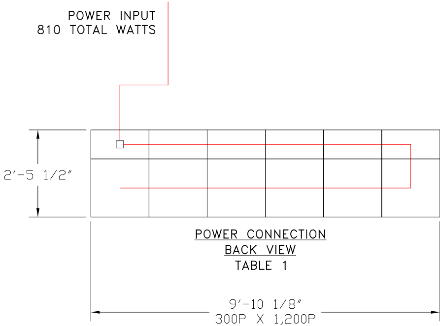
CST-102E, 2.5MM 300H X 1,200L INDOOR FRONT SERVICE SINGLE-FACE FULL-COLOR DIGITAL VIDEO DISPLAY POWER CONNECTION BACK VIEW
