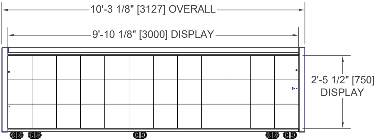
(1) CST-102E, 2.5MM 300H X 1,200L FRONT VIEW
