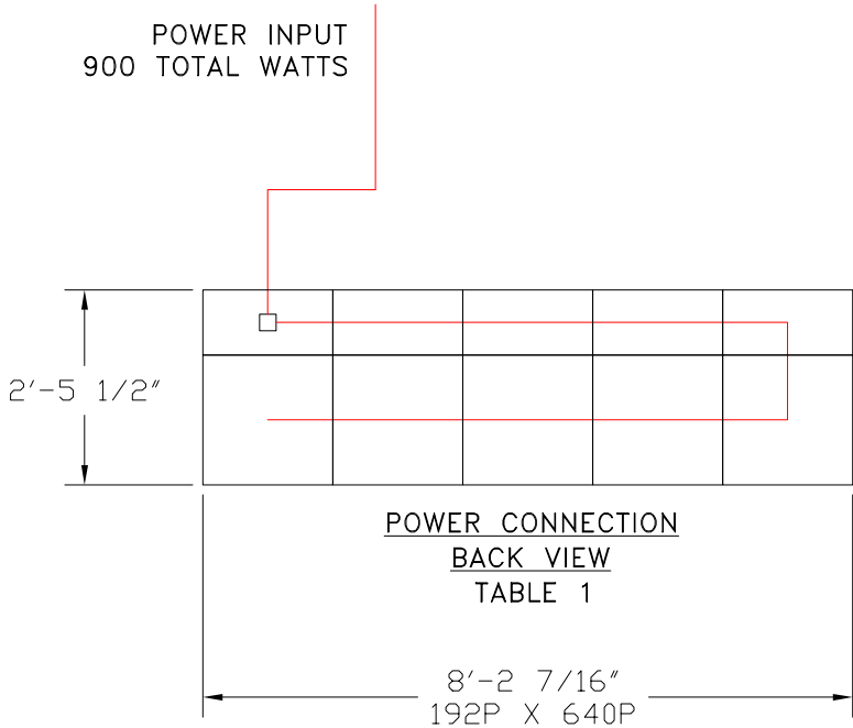
CST-083E, 3.9MM 192H X 640L INDOOR FRONT SERVICE SINGLE-FACE FULL-COLOR DIGITAL VIDEO DISPLAY POWER CONNECTION BACK VIEW
