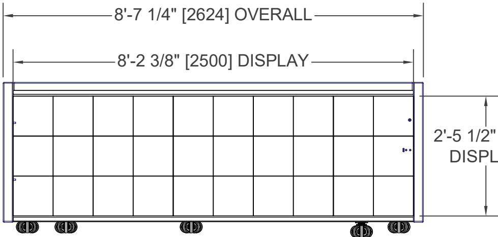
(1) CST-083E, 3.9MM 192H X 640L FRONT VIEW
