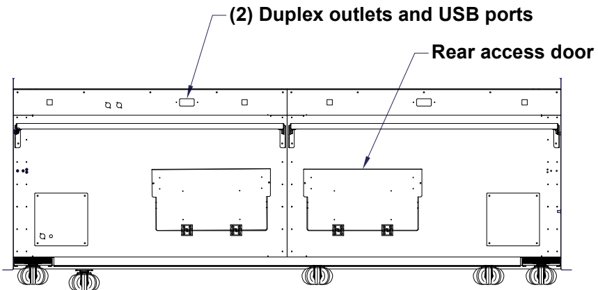
BACK VIEW (WITHOUT PADDING)
