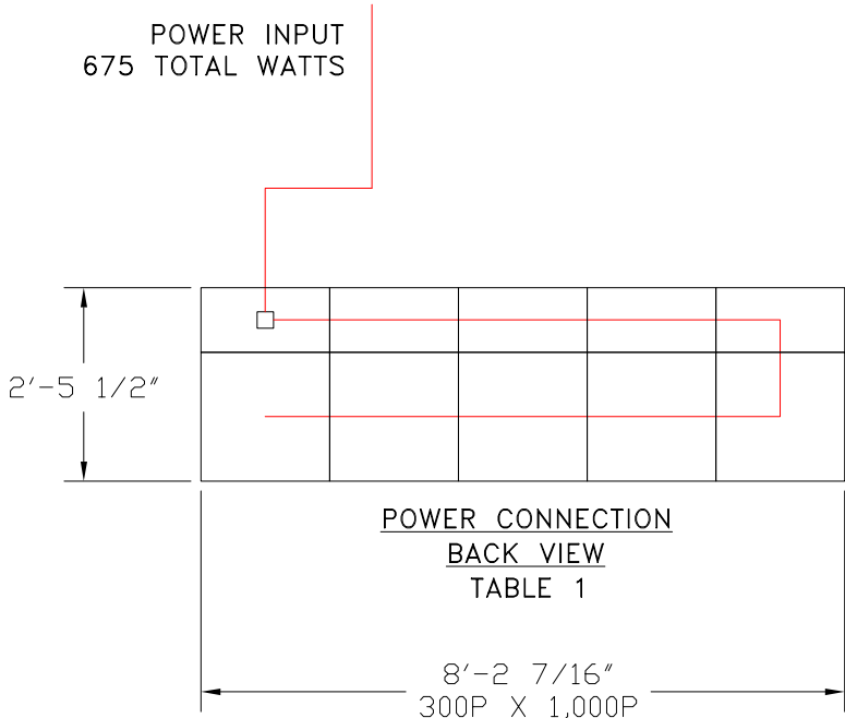
CST-082E, 2.5MM 300H X 1,000L INDOOR FRONT SERVICE SINGLE-FACE FULL-COLOR DIGITAL VIDEO DISPLAY POWER CONNECTION BACK VIEW
