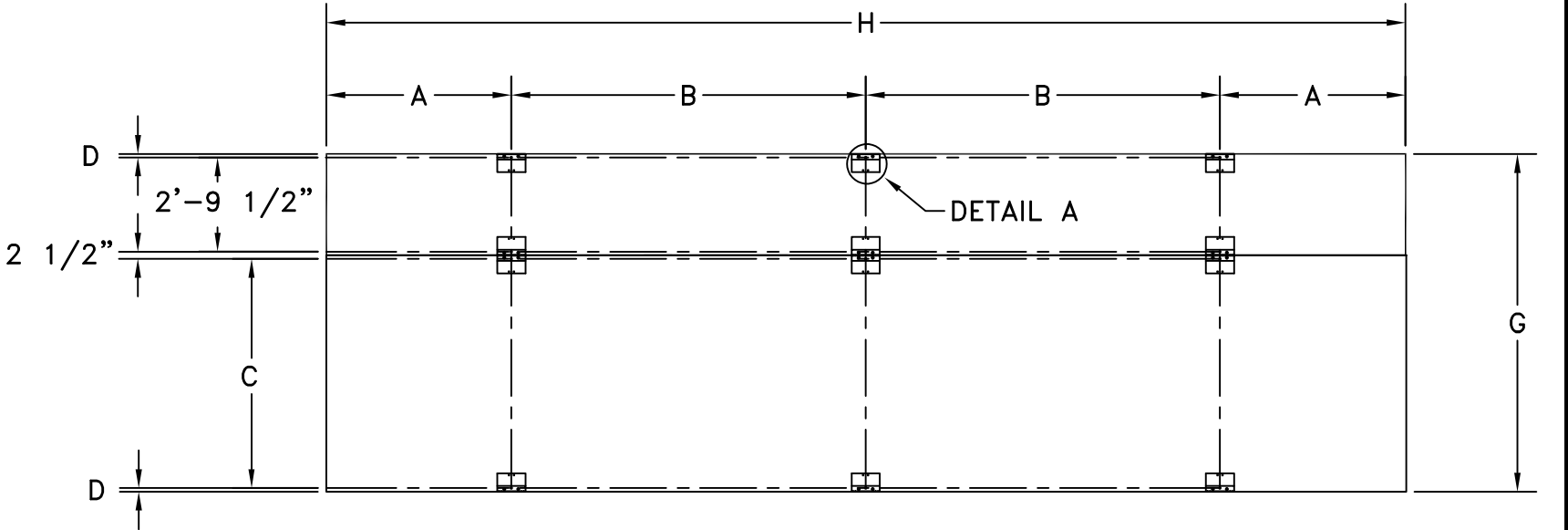
HANGER BRACKET DETAIL BACK VIEW
