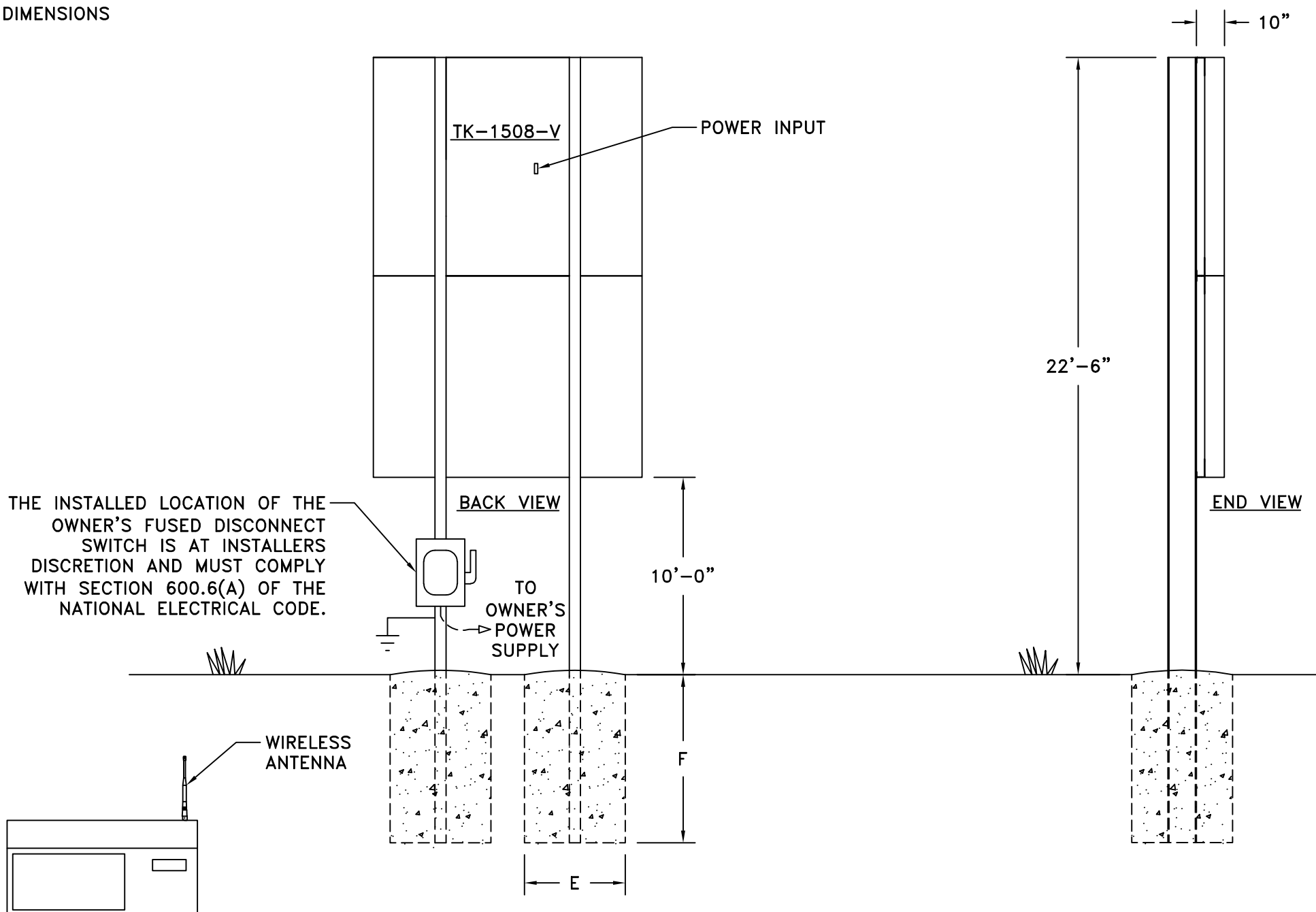
SCBD CONTROL WIRELESS SHOWN
