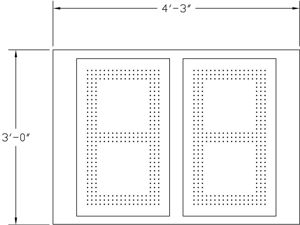
T-830-DISPLAY SINGLE-POLE INSTALLATION
