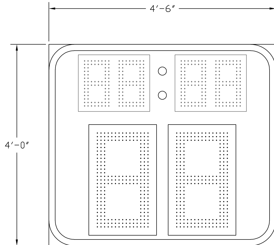
T-0448-06-DISPLAY GAME CLOCK/PLAY CLOCK DISPLAY TOP: GAME CLOCK USING 12"H AMBER LED DIGITS BOTTOM: PLAY CLOCK USING 24"H AMBER LED DIGITS
