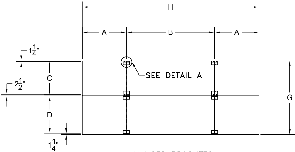
HANGER BRACKETS BACK VIEW
