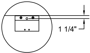
STANDARD J HANGER BRACKET
