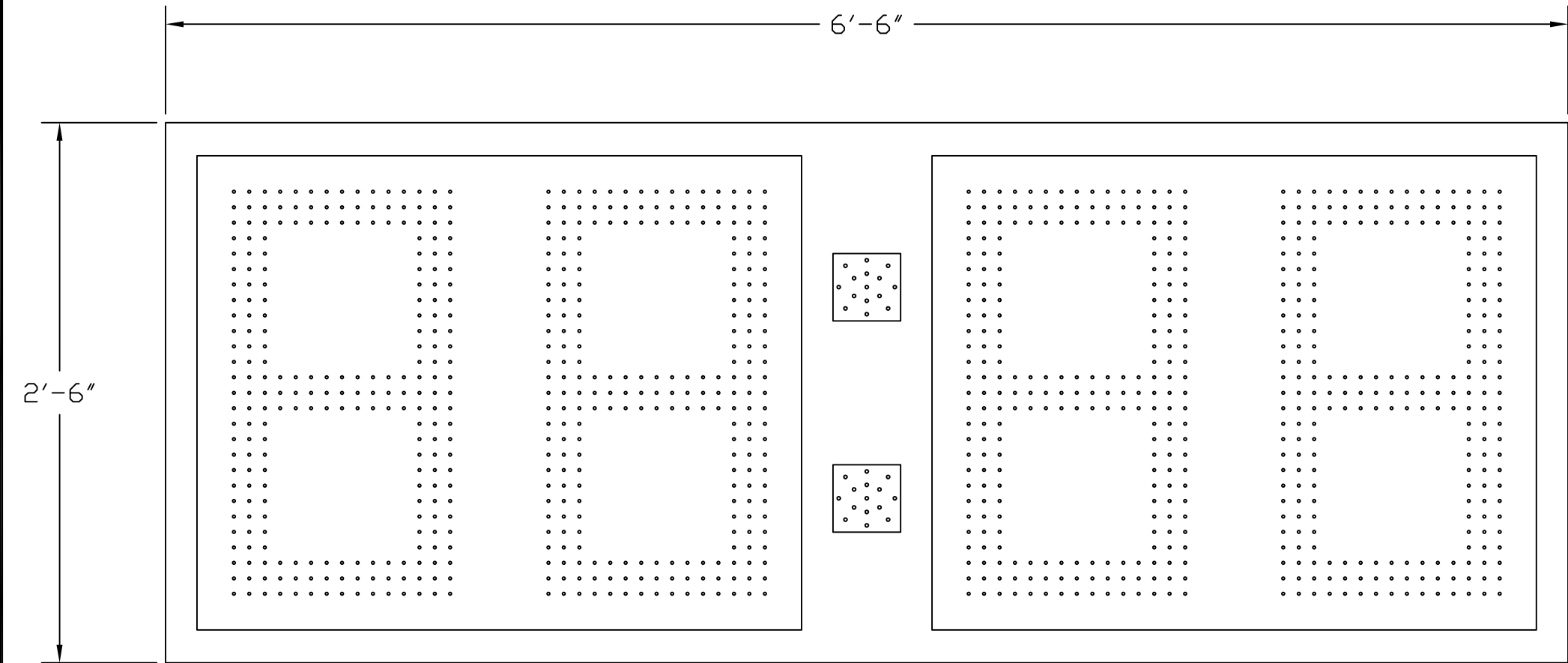
PT-063024-06 (OUTDOOR 4-DIGIT PITCH TIMER USING 24"H AMBER LED DIGITS WITH AMBER LED LIT COLON)
