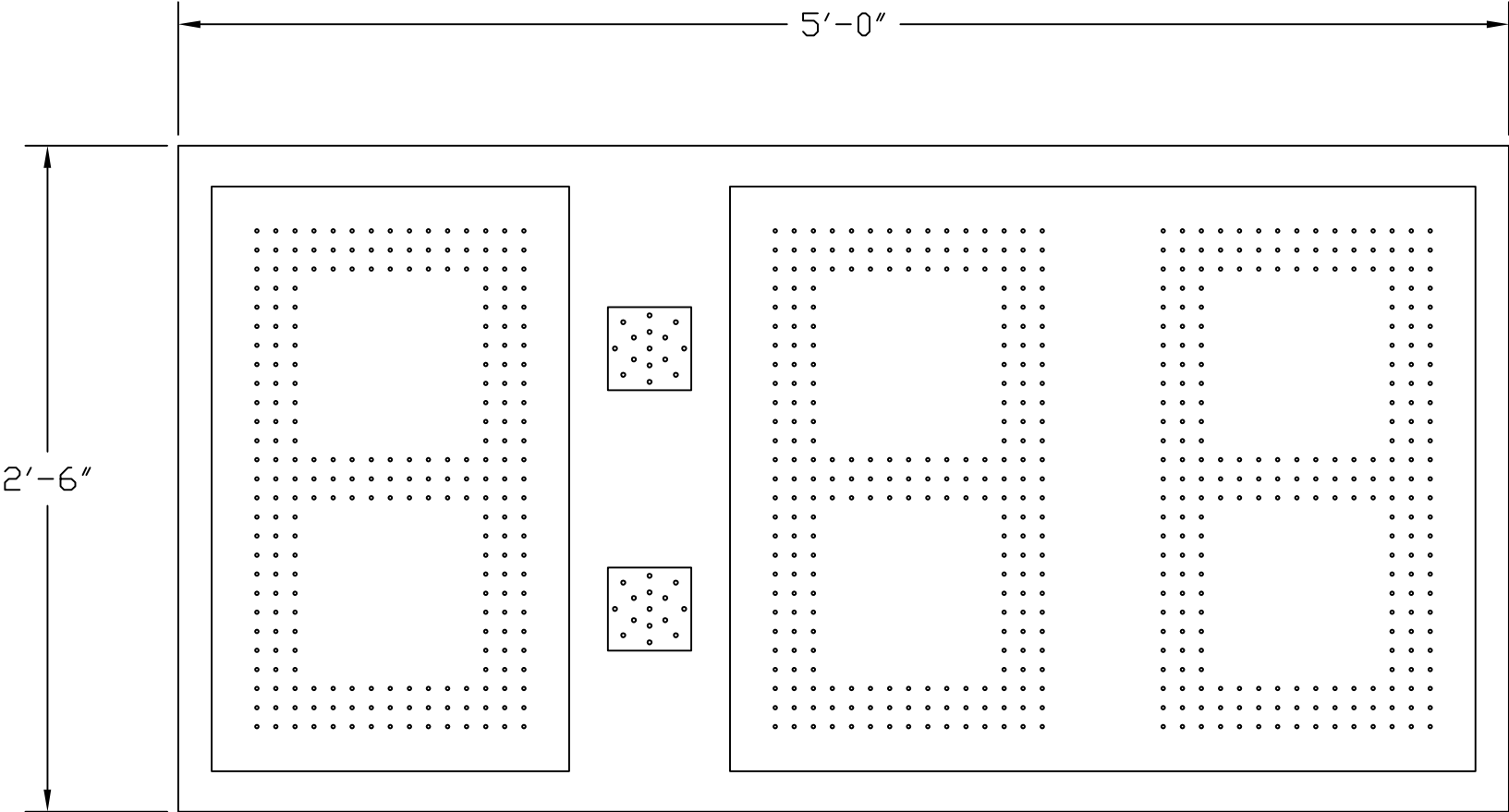
PT-053024 OUTDOOR 3-DIGIT PITCH TIMER USING 24"H AMBER LED DIGITS WITH AMBER LED LIT COLON
