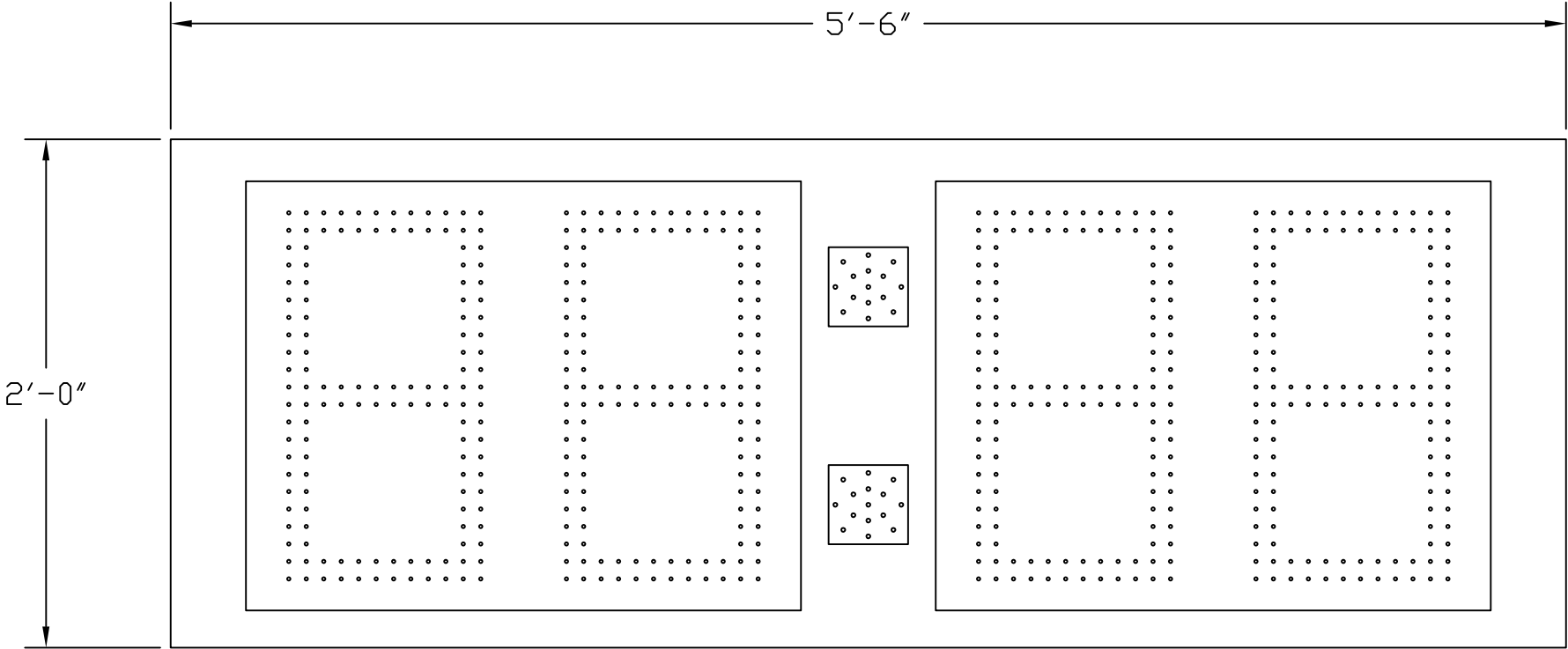
PT-052418-06 (OUTDOOR 4-DIGIT PITCH TIMER USING 18"H AMBER LED DIGITS WITH AMBER LED LIT COLON)
