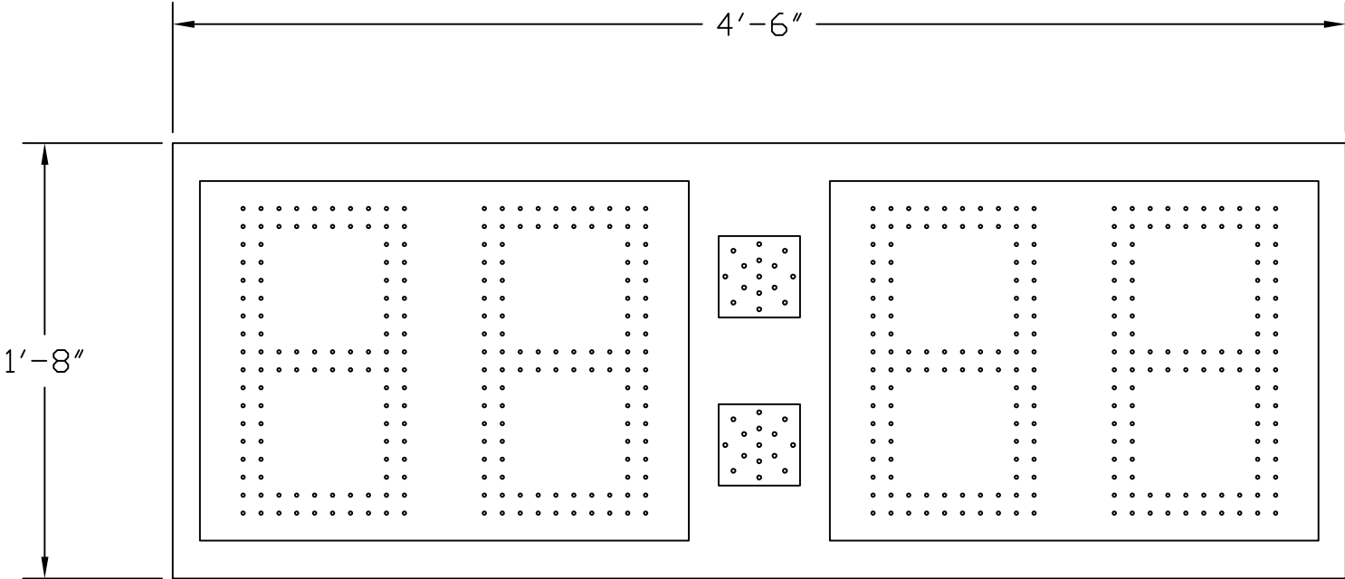
PT-042015-06 (OUTDOOR 4-DIGIT PITCH TIMER USING 15"H AMBER LED DIGITS, AMBER LED LIT COLON)
