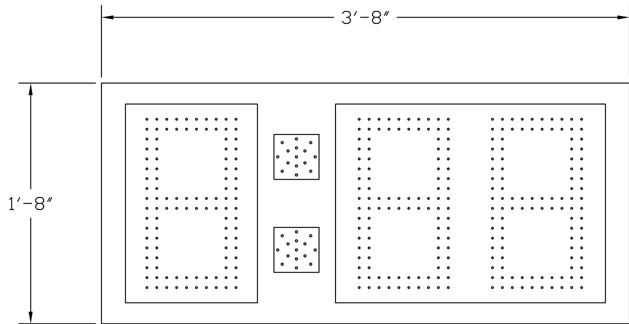
PT-032015-08 (OUTDOOR 3-DIGIT PITCH TIMER USING 15"H AMBER LED DIGITS, AMBER LED LIT COLON)
