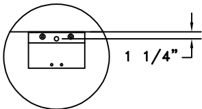
STANDARD J BRACKET
