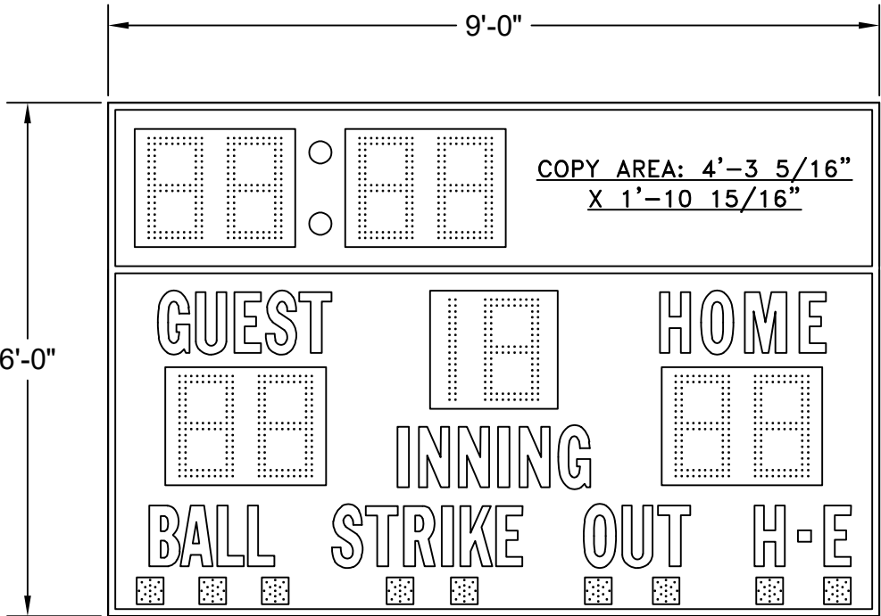
MP-7109T4 BASEBALL ARRANGEMENT
