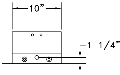
DETAIL A "J" BRACKET
