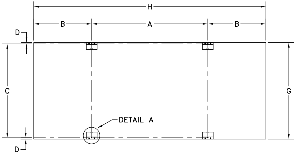
HANGER BRACKET DETAIL (BACK VIEW)
