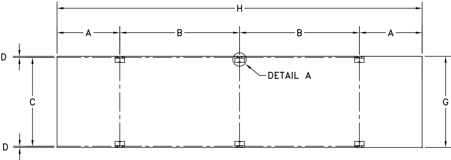
HANGER BRACKET DETAIL BACK VIEW
