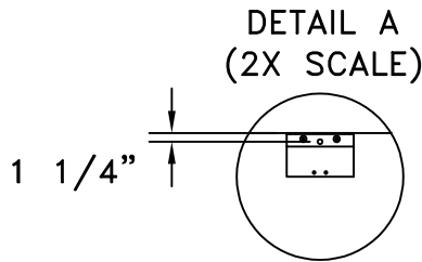
STANDARD "J" BRACKET DETAILS
