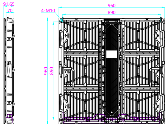
CABINET DRAWING
