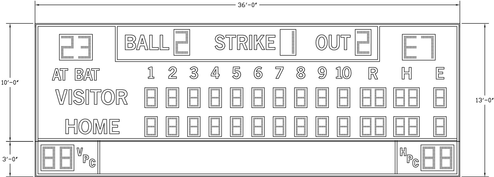
BA-7136PC (24"H DIGITS MOVED TO THE ENDS OF PITCH COUNT SECTION, ADDED TRIM)
