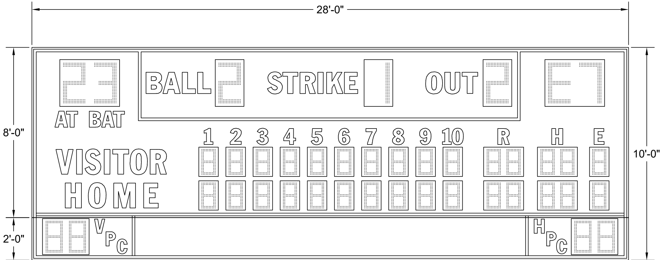
BA-7128PC (18"H DIGITS MOVED TO THE ENDS OF PITCH COUNT SECTION, ADDED TRIM)
