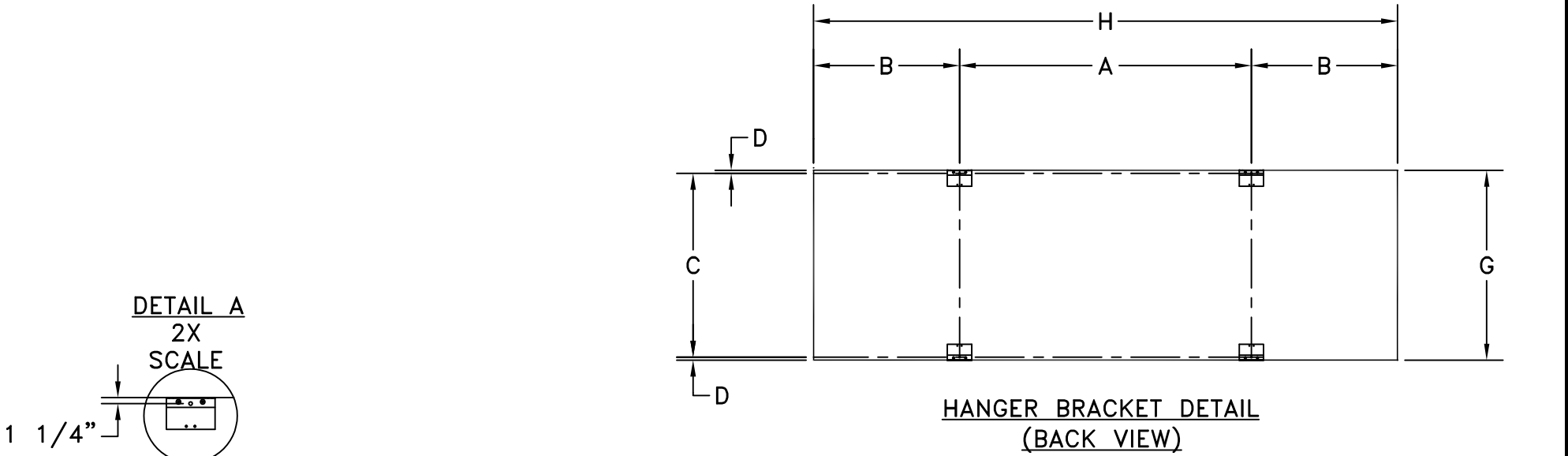
STANDARD "J" HANGER BRACKET
