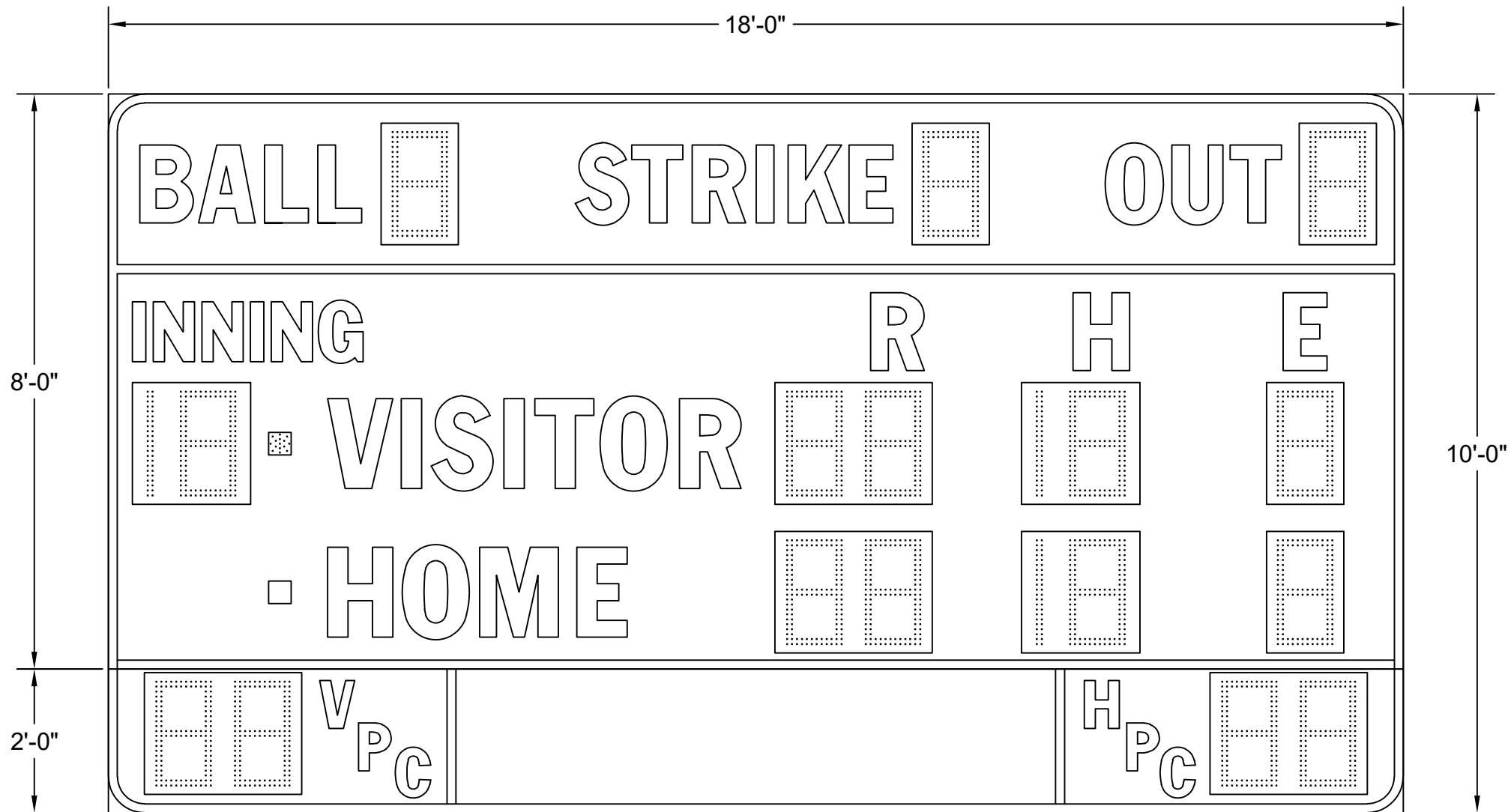
BA-7118PC (18"H DIGITS MOVED TO ENDS OF PITCH COUNT SECTION, ADDED TRIM)
