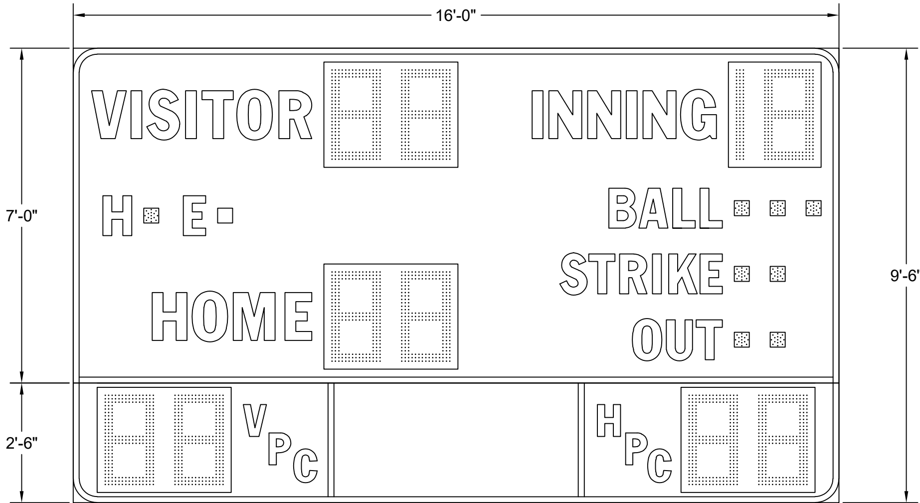
BA-7116PC (24"H DIGITS MOVED TO THE ENDS OF PITCH COUNT SECTION, ADDED TRIM)
