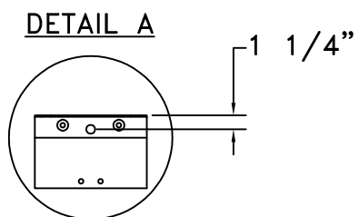
STANDARD J BRACKET
