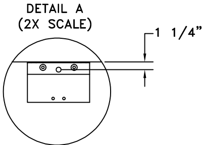
STANDARD J BRACKET
