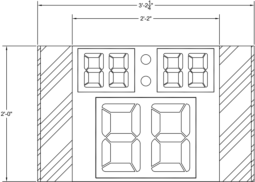
ST-1425-3S-4 3-SIDED LED BAR DIGIT INDOOR SHOT TIMER/GAME CLOCK FACE 1 SHOWN, OTHERS TYPICAL
