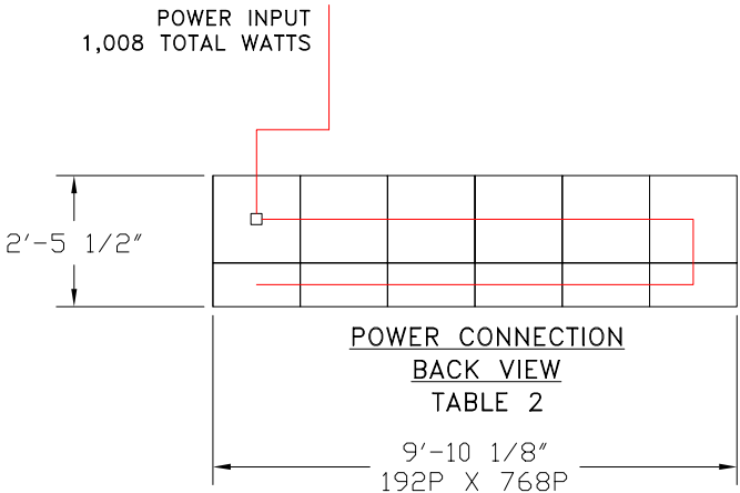
CST-1003-4, 3.9MM 192H X 768L INDOOR FRONT SERVICE SINGLE-FACE FULL-COLOR DIGITAL VIDEO DISPLAY POWER CONNECTION BACK VIEW
