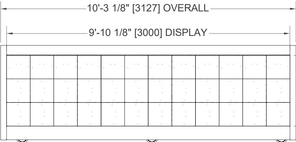
(1) CST-1003, 3.9MM 192H X 768L FRONT VIEW
