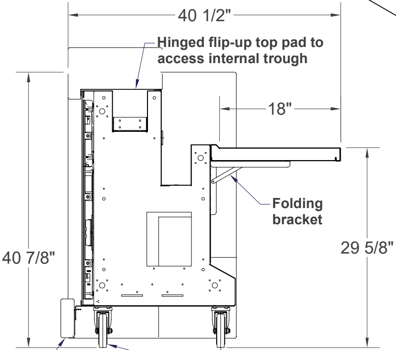
SIDE VIEW SIDE PAD REMOVED
