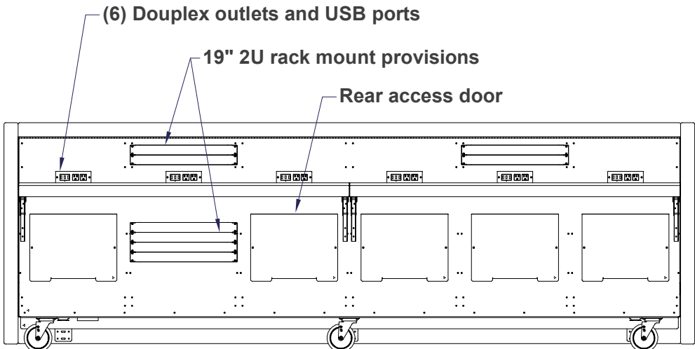
BACK VIEW
