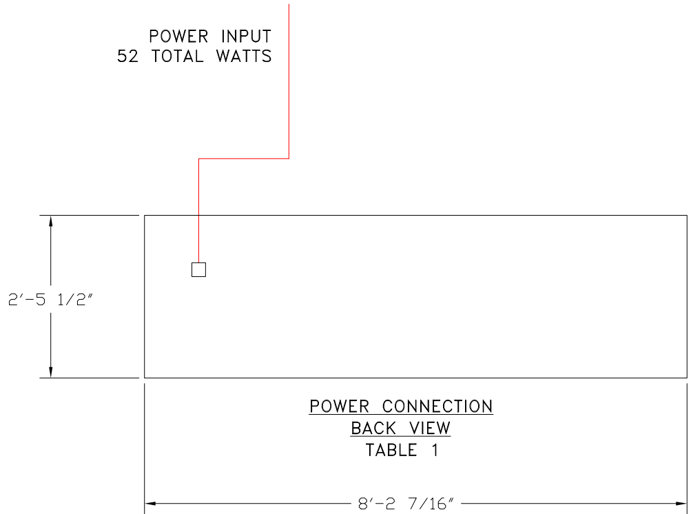
CST-08RI-4, REAR ILLUMINATED COURT SIDE TABLE POWER CONNECTION BACK VIEW
