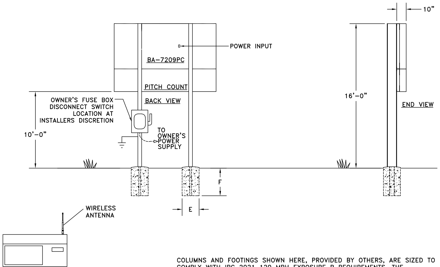
SCBD CONTROL WIRELESS SHOWN
