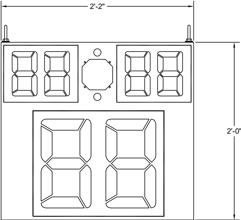
ST-1425-4-2S 2-SIDED LED BAR DIGIT INDOOR SHOT TIMER/GAME CLOCK FACE 1 SHOWN, FACE 2 TYPICAL
