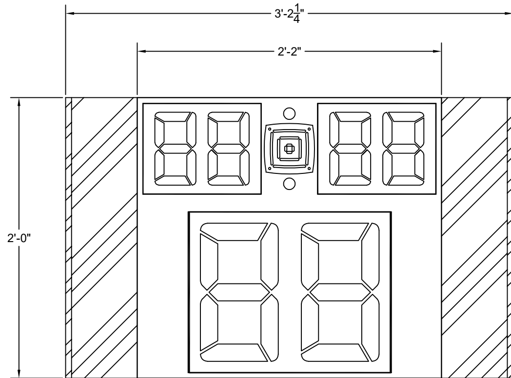
ST-1425-3S-4 3-SIDED LED BAR DIGIT INDOOR SHOT TIMER/GAME CLOCK FACE 1 SHOWN, OTHERS TYPICAL
