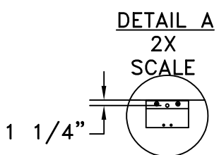
STANDARD "J" HANGER BRACKET
