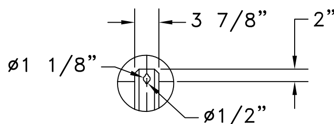
DETAIL A MOUNTING BRACKET
