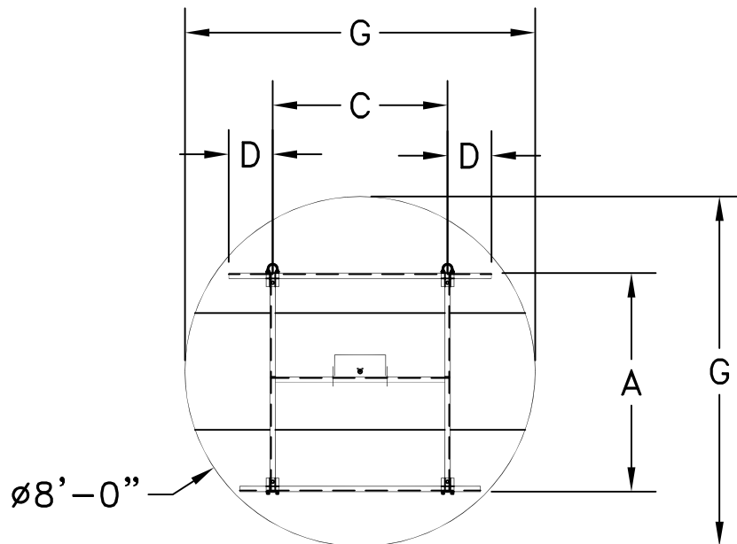
HANGER BRACKET DETAIL BACK VIEW
