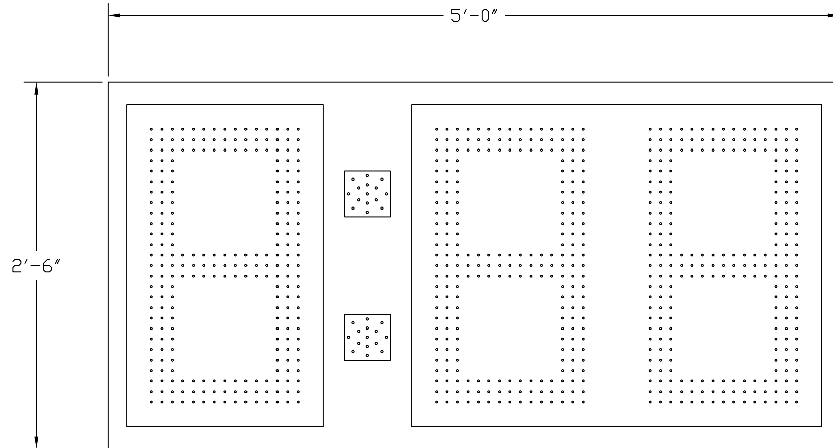
PT-053024-2 OUTDOOR 3-DIGIT PITCH TIMER USING 24"H AMBER LED DIGITS WITH AMBER LED LIT COLON
