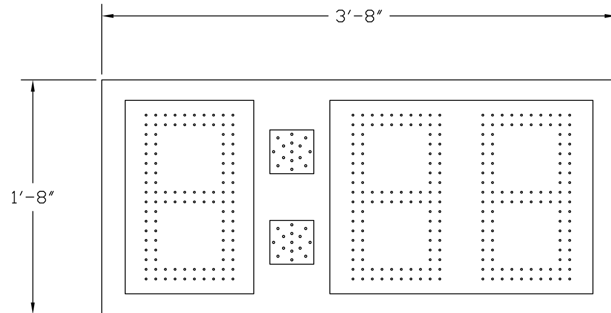
PT-032015-08-2 OUTDOOR 3-DIGIT PITCH TIMER USING 15"H AMBER LED DIGITS, AMBER LED LIT COLON
