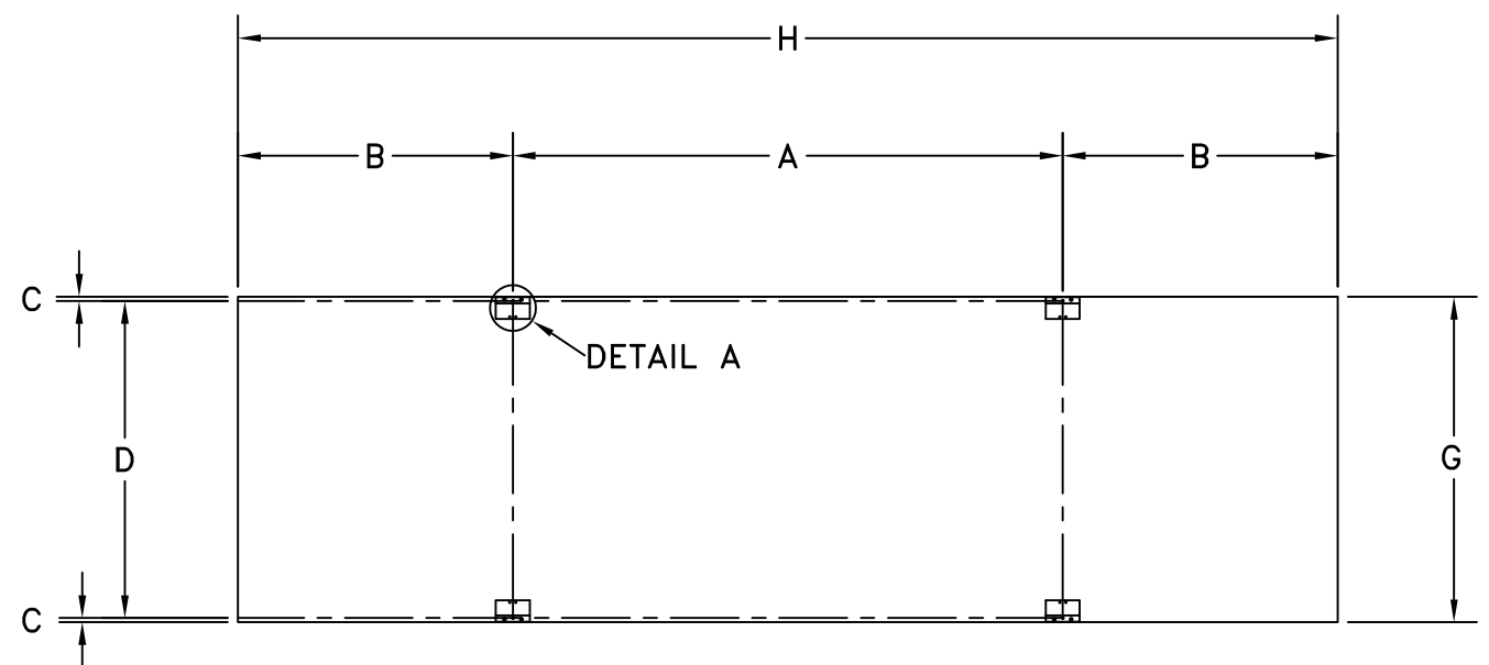
HANGER BRACKETS BACK VIEW
