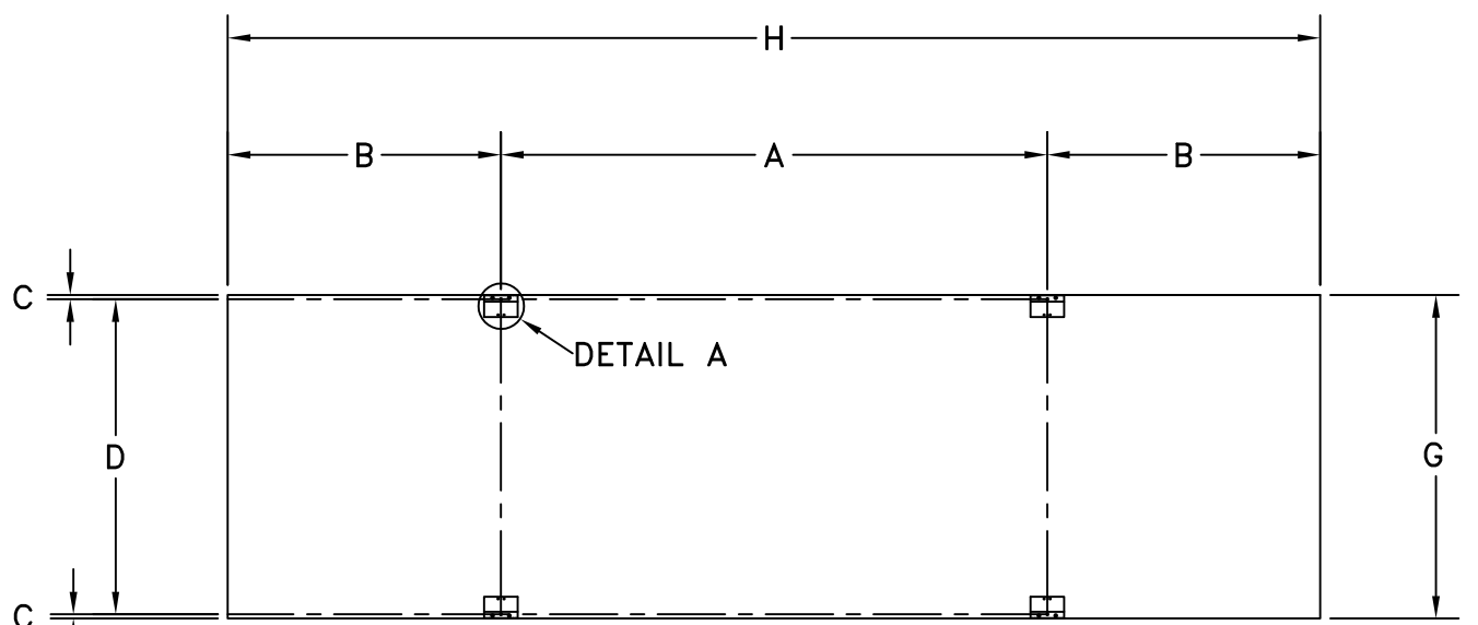
HANGER BRACKETS BACK VIEW
