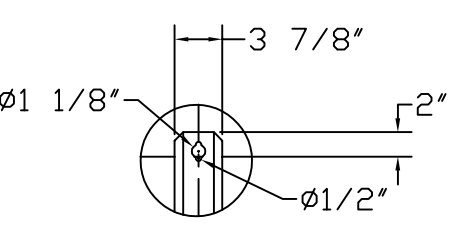
DETAIL A MOUNTING BRACKET
