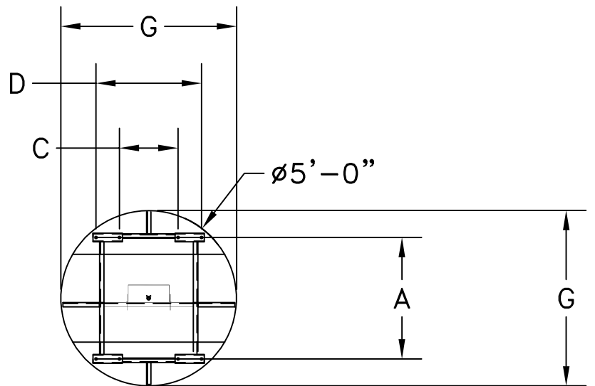
HANGER BRACKET DETAIL BACK VIEW
