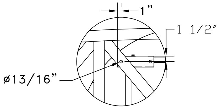
DETAIL A "J" BRACKET 1/4" PLATE STEEL
