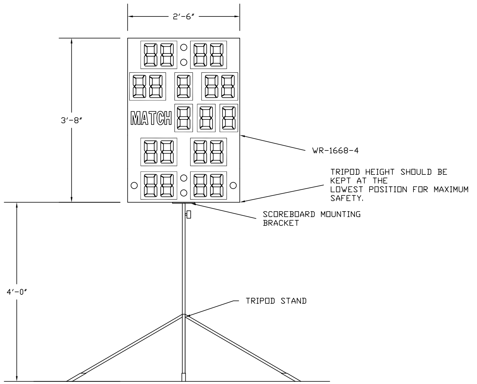
FRONT VIEW
