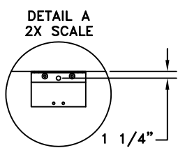
STANDARD "J" BRACKET 1/4" STEEL
