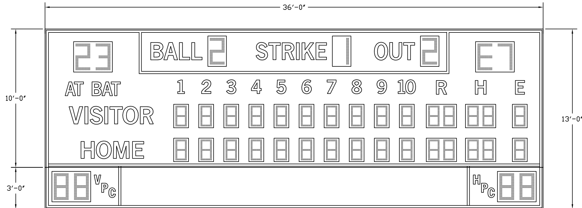
BA-7136PC-2 (24"H DIGITS MOVED TO THE ENDS OF PITCH COUNT SECTION, ADDED TRIM)
