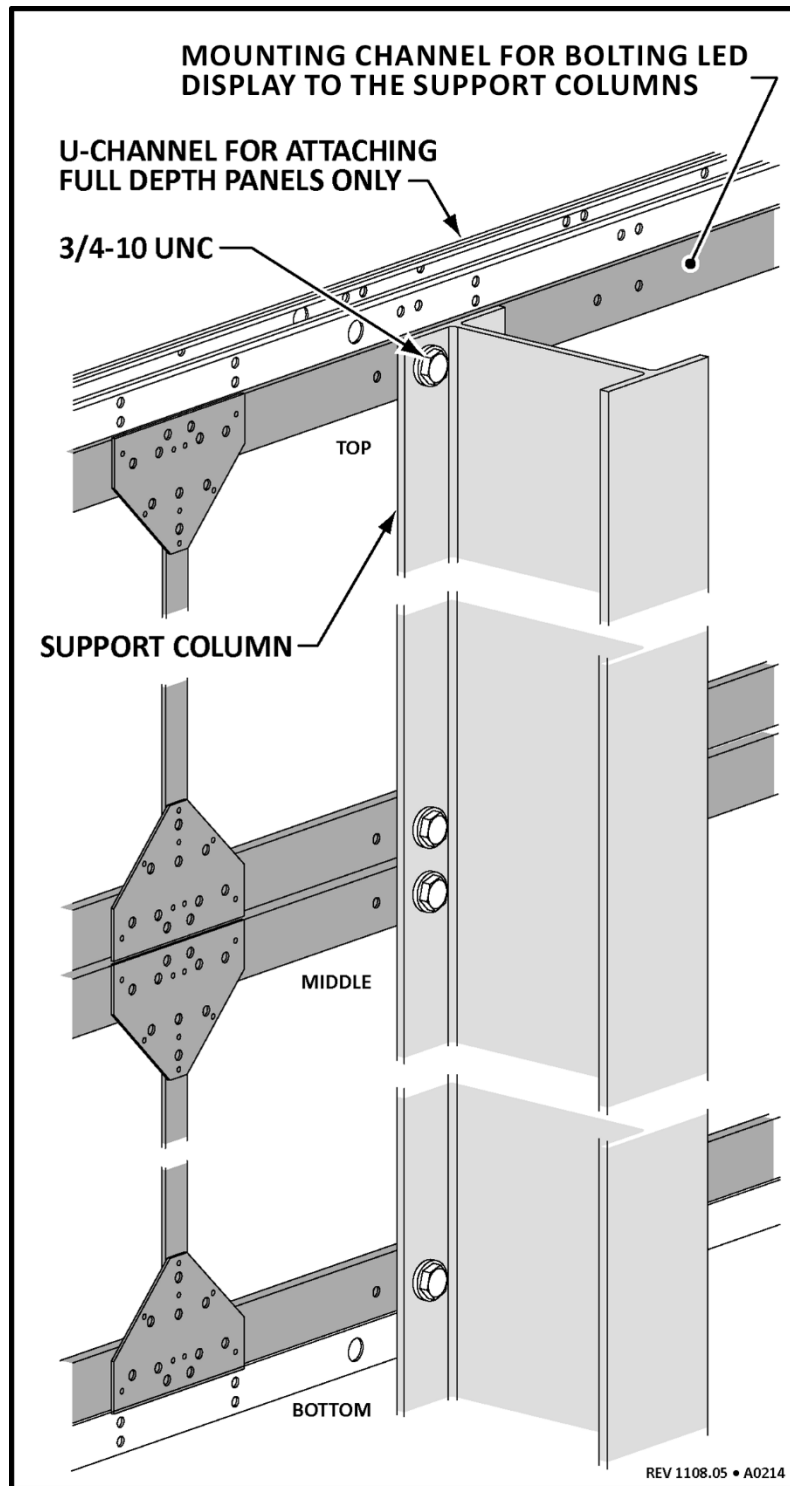
FIGURE 16 — BOLTED
