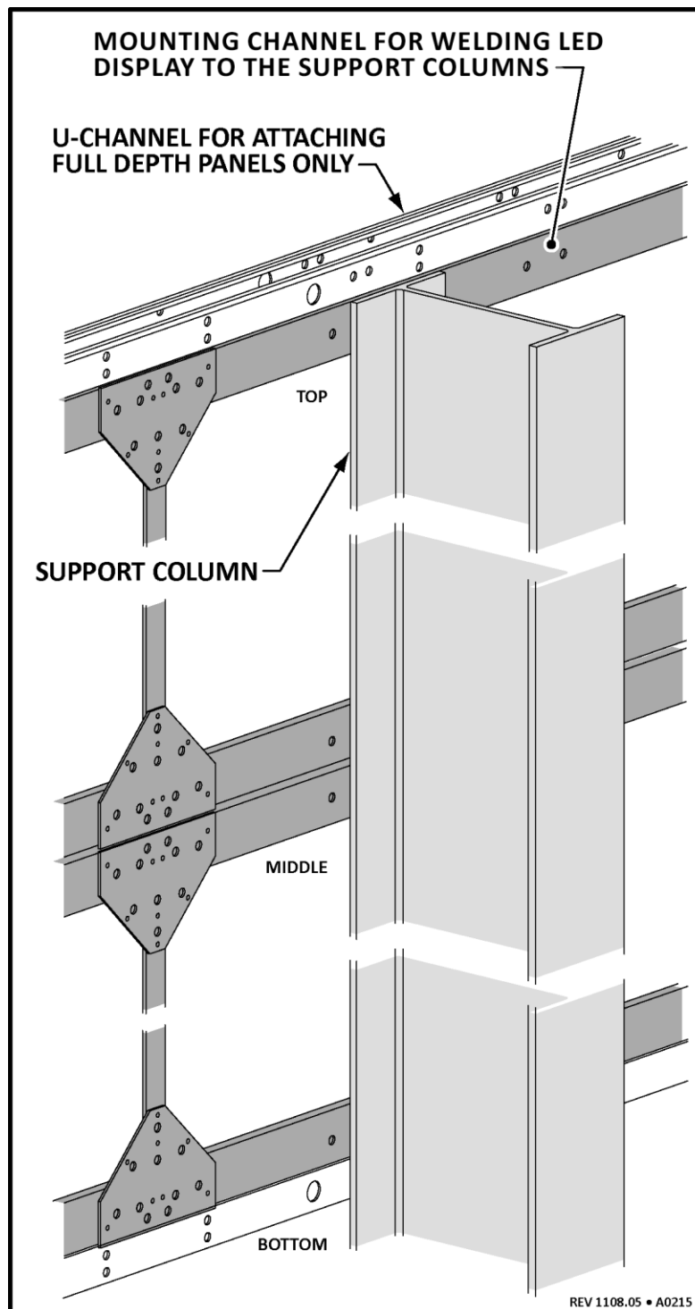
FIGURE 18 — WELDING
