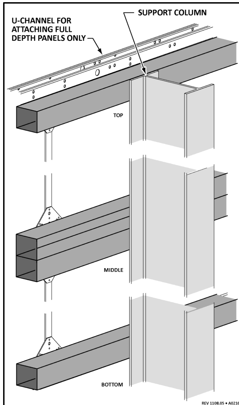
FIGURE 17 — STRINGER
