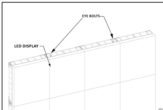
FIGURE 12 — LIFTING BRACKETS
