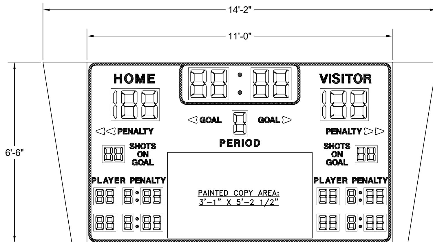
HK-1880A-4 FOUR-SIDED HOCKEY SCOREBOARD FACE 1 OF 4 SHOWN - ALL OTHERS TYPICAL
